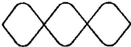
SSB SIGNAL, TONE INPUT WITH PROPER CARRIER INSERTED 100% MODULATED
